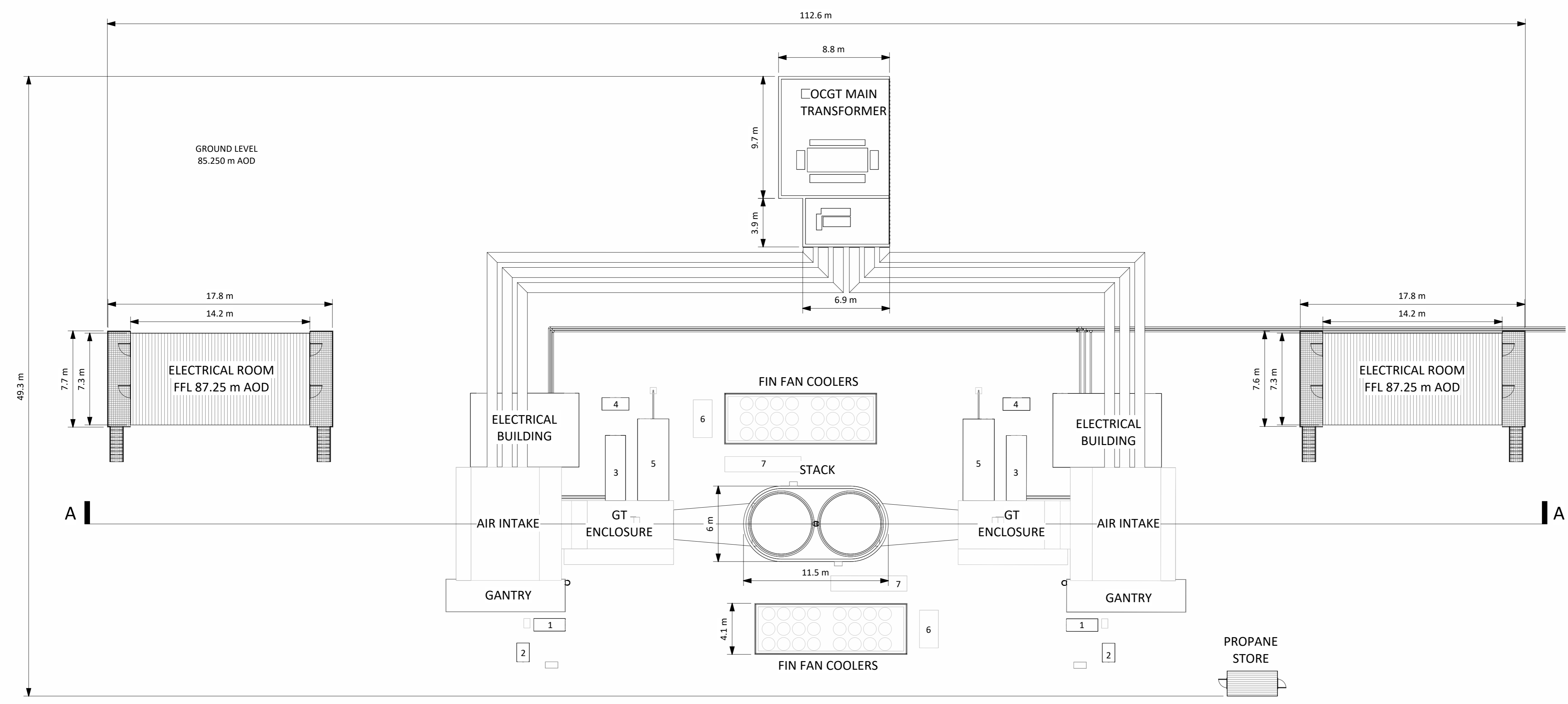
1 OCGT Plan 85.250m AOD 1 : 200
